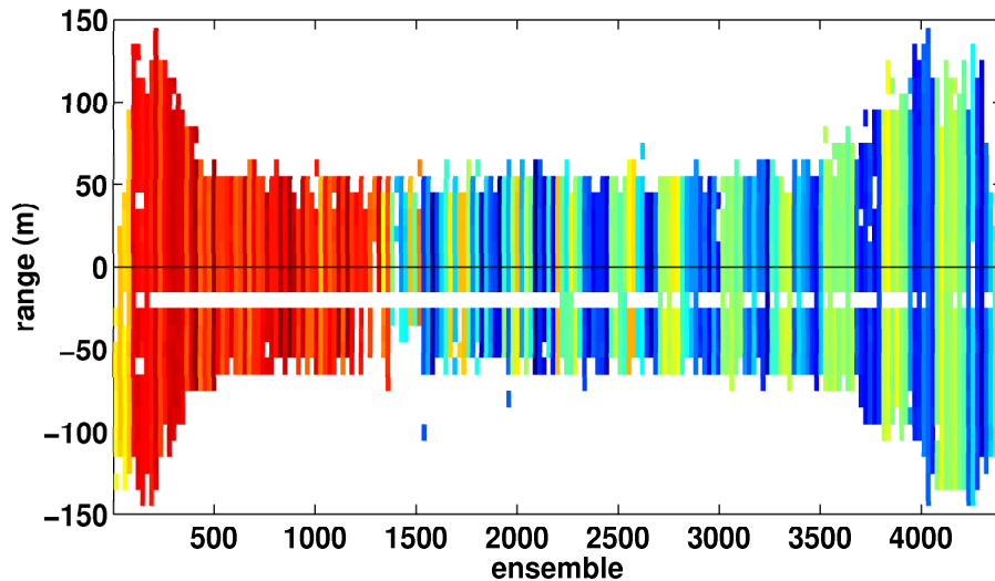
Figure 17: Typical depth ranges of upward and downward looking BB300 during LADCP cast (here station # 16).
